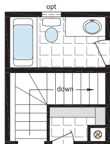
Proposed Stair Location for Optional Foundation Model
