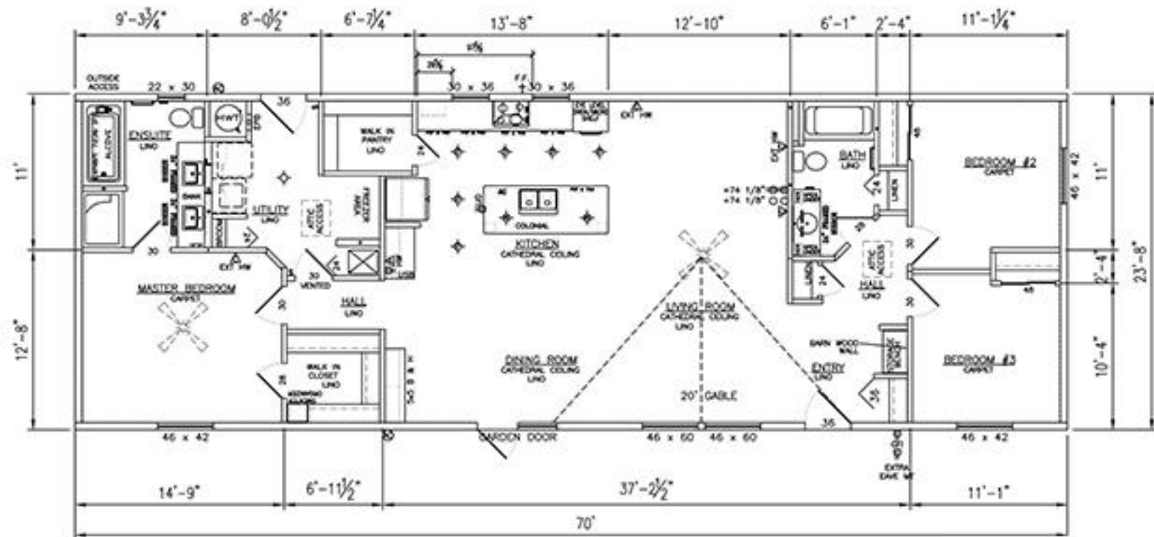
2295 Floorplan
